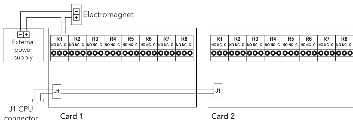
Wiring diagram of supervised relay cards
