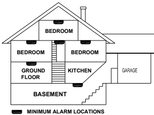
Fig. 2 – Multi-storey dwelling
