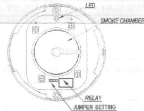
Fig. 3 Schematic of detector structure When front cover is open
