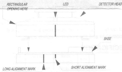
Fig. 2 Mating detector head onto base
