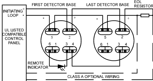
NOTE: IF REMOTE INDICATOR IS NOT USED, POLARITY TO DETECTOR MAY BE REVERSED. Fig. 1.a Installing the 2-wire multiple station smoke detector base
