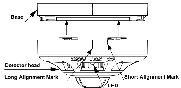
Fig. 3: Fitting the detector to the base
