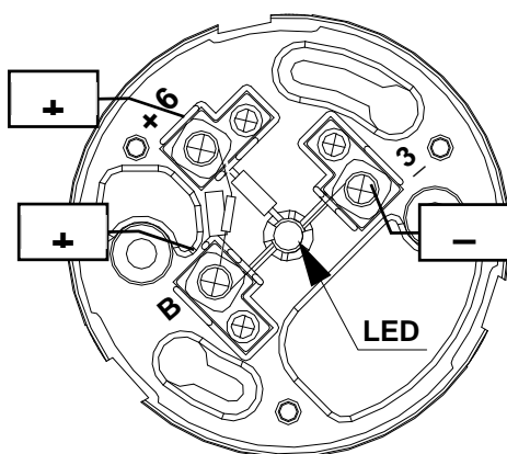
Fig. 1: 681 wiring connections
